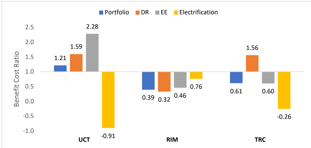
Figure 4-20: Benefit-Cost Ratios for DSM Portfolio Categories
